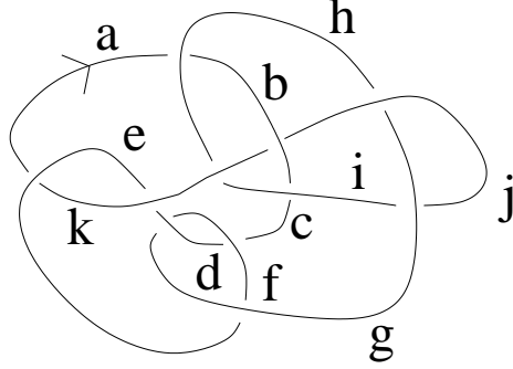
FIGURE 3. The Conway knot 11_{401} and the Kinoshita–Terasaka knot 11_{409} .
