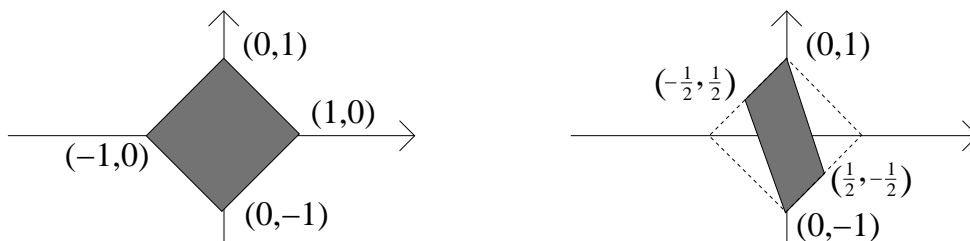
FIGURE 8. Alexander norm ball and Thurston norm ball for Dunfield's link.
