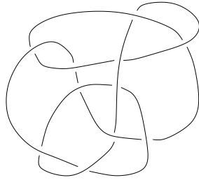
FIGURE 1. The Conway knot 11_{401} and a Seifert surface of genus 3 (from [Ga84]).
