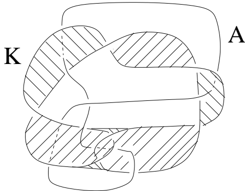
FIGURE 5. Seifert surface for K \subset S^3 \setminus K \cup A .
