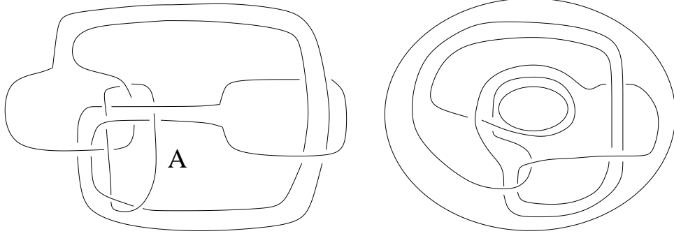
FIGURE 4. Knot 6_1 with choice of A and considered as a knot in the solid torus X(A) .
