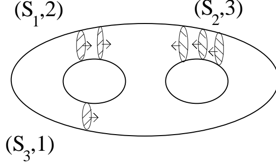
FIGURE 2. Weighted surface in a handlebody.
