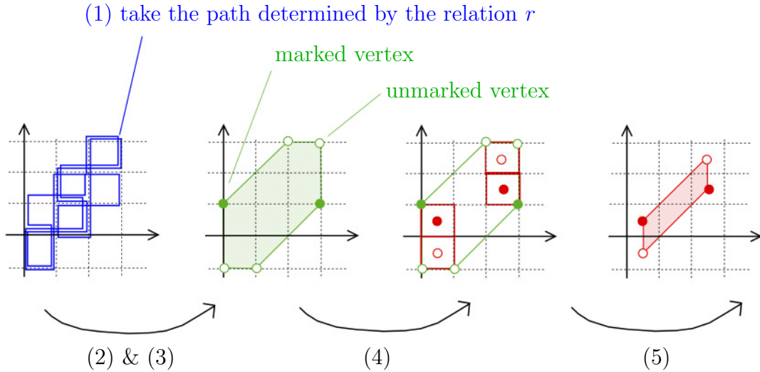
FIGURE 1. The marked polytope \mathcal{M}_\pi for Dunfield's example (labels on arrows correspond to steps in the above algorithm).
