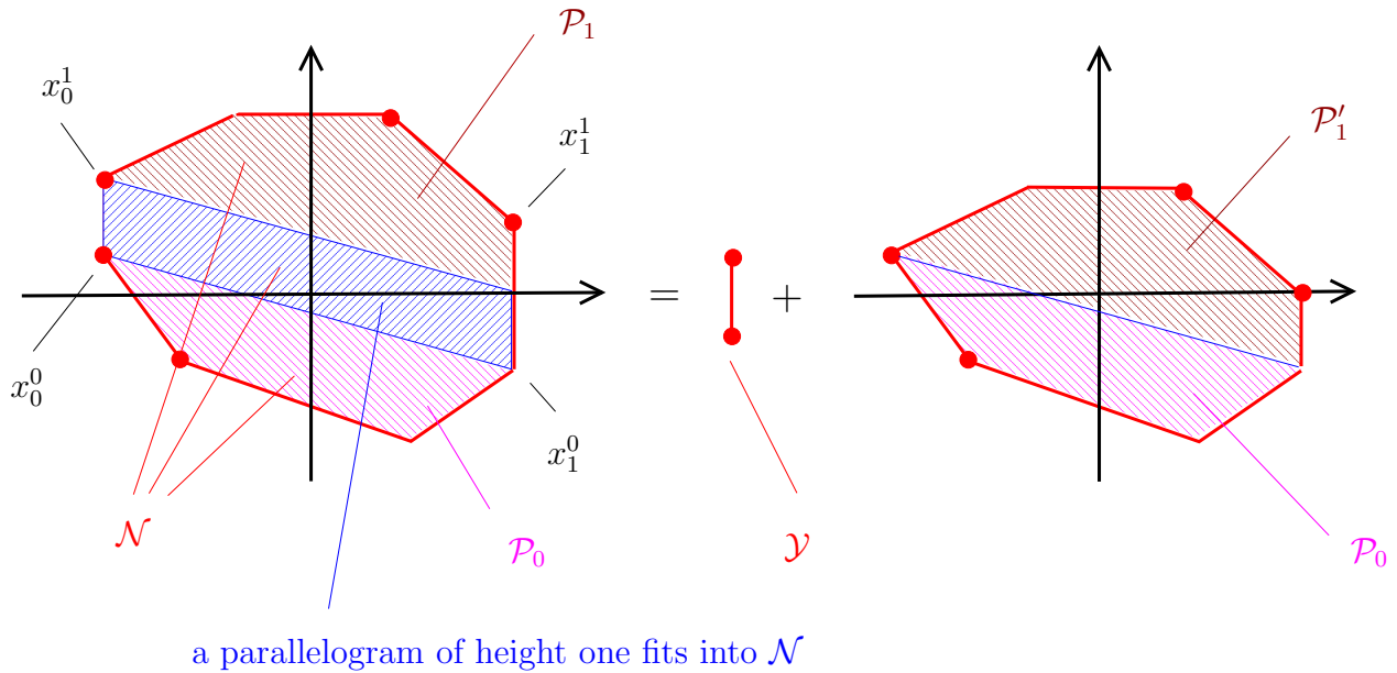
FIGURE 4. Subtracting \mathcal{Y} .
