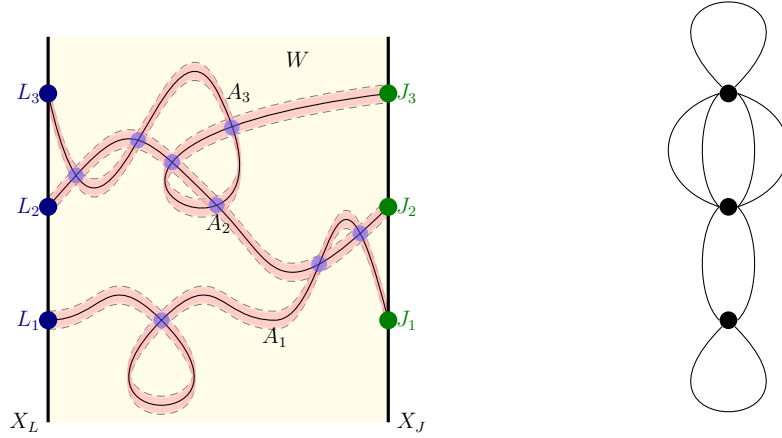
FIGURE 1. Left: an example of an immersed concordance. The picture is a sketch in dimension 2. The annuli are represented by curves and the links are represented as points. The manifold W is the part of the picture outside the neighbourhood of the annuli. The dashed curves represent P . Right: the corresponding graph \Gamma (the labelling of the edges is not drawn).
