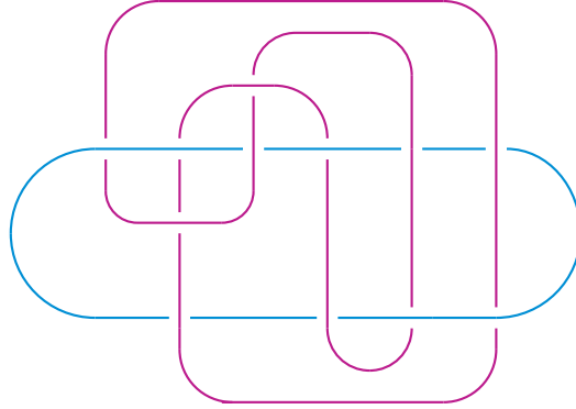
FIGURE 5. The link L12n1320 .
