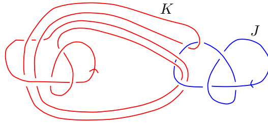
FIGURE 4. A band-claspings of two trefoils.
