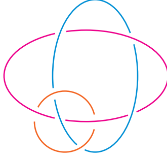
FIGURE 6. The link L8a16 .
