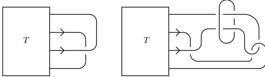
FIGURE 7. Left: the box denotes a tangle T such that the diagram is an unknotting number one knot with the unknotting crossing isolated. Right: replace the strands outside the box as shown to get a 2-component link L_T with unknotted components and weak splitting number one.
