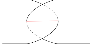
FIGURE 2. Clasp singularities between two surfaces.
