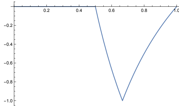
FIGURE 2. \Upsilon_{T(3,7)-T(4,5)}(t)/t
